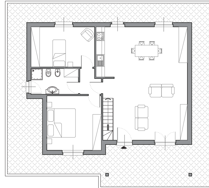
Piano Terra
